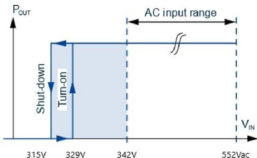
Fig. 7-1: Shut-down behavior, definitions
