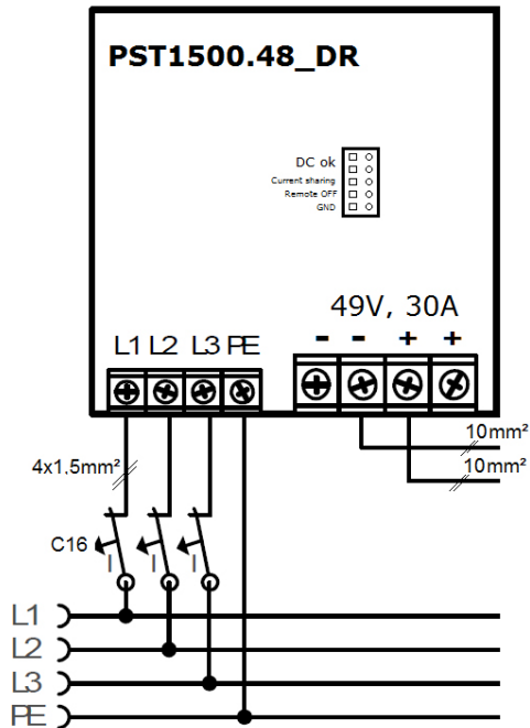
Single Installation
