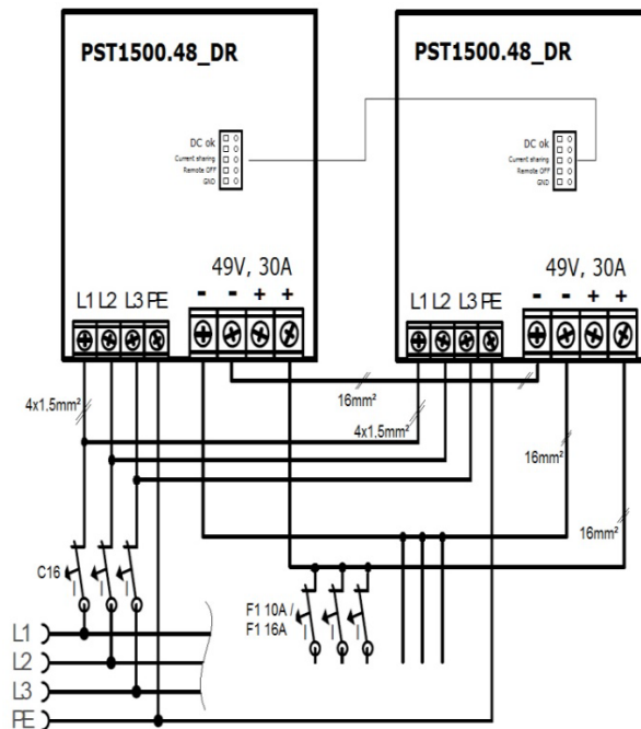
Parallel operation
